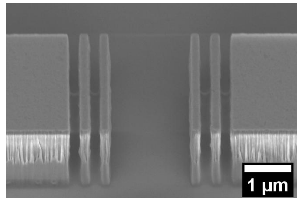
Fig. 2: Bragg reflectors for visible light in a Si 3 N 4 waveguide for integration into a MOEMS.
